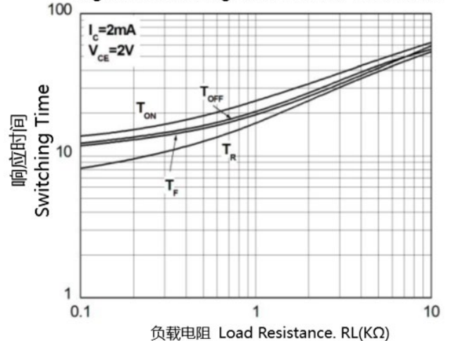
Figure6. Switching Time vs Load Resistance
