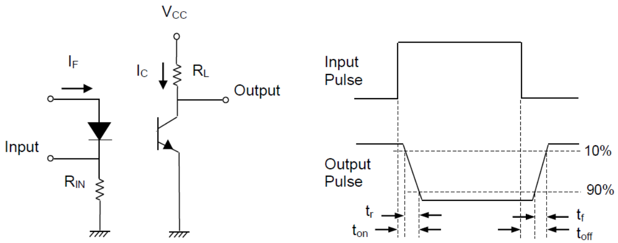
Fig7. Switching Time Test Circuit & Waveforms
