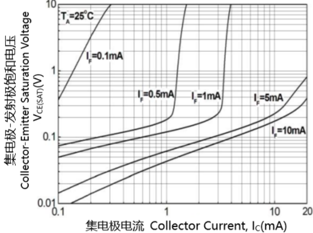
Figure5. Collector-Emitter Saturation Voltage vs Collector Current
