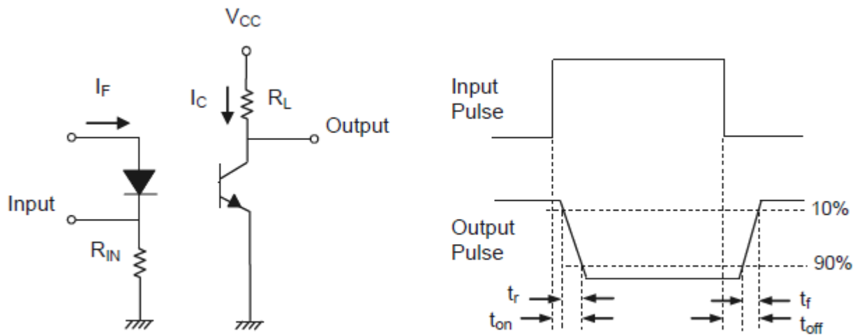
Fig7. Switching Time Test Circuit &amp; Waveforms
